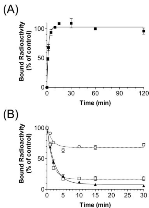
Fig. 2. [ ^3\text{H} ]ETB-TBOA binding to and dissociation from rat brain crude membranes. A, association of 10 nM [ ^3\text{H} ]ETB-TBOA at room temperature. Bound radioactivities were normalized to the value at 60 min. B, dissociation of 10 nM [ ^3\text{H} ]ETB-TBOA in the presence of 1 mM L-glutamate ( \circ ), 10 mM L-glutamate ( \square ), or 10 \mu\text{M} TFB-TBOA ( \blacktriangle ) after a 30-min association. Data represent the mean \pm S.E.M. from three separate experiments.
