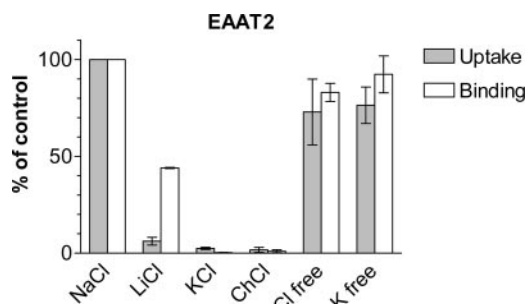
Fig. 6. Effects of ions on [ ^3\text{H} ]ETB-TBOA binding to EAAT2-expressing cell membranes ( \square ) and [ ^{14}\text{C} ]glutamate uptake by EAAT2-expressing cells ( \blacksquare ). Data represent mean \pm S.E.M. of at least three separate experiments.
