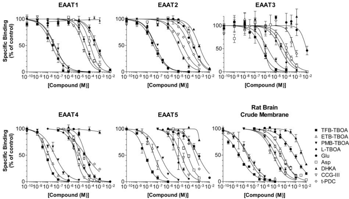
Fig. 7. Displacement of [ 3 H]ETB-TBOA binding by drugs known to interact with EAATs in EAAT-expressing cell membranes and rat brain crude membranes. Specific binding was normalized to the control (100%). Nonspecific binding was determined in the presence of 10 \mu M TFB-TBOA. Data represent mean \pm S.E.M. of at least three separate experiments. The concentration of [ 3 H]ETB-TBOA used and the K_i values of inhibitors for each preparation are summarized in Table 2.
