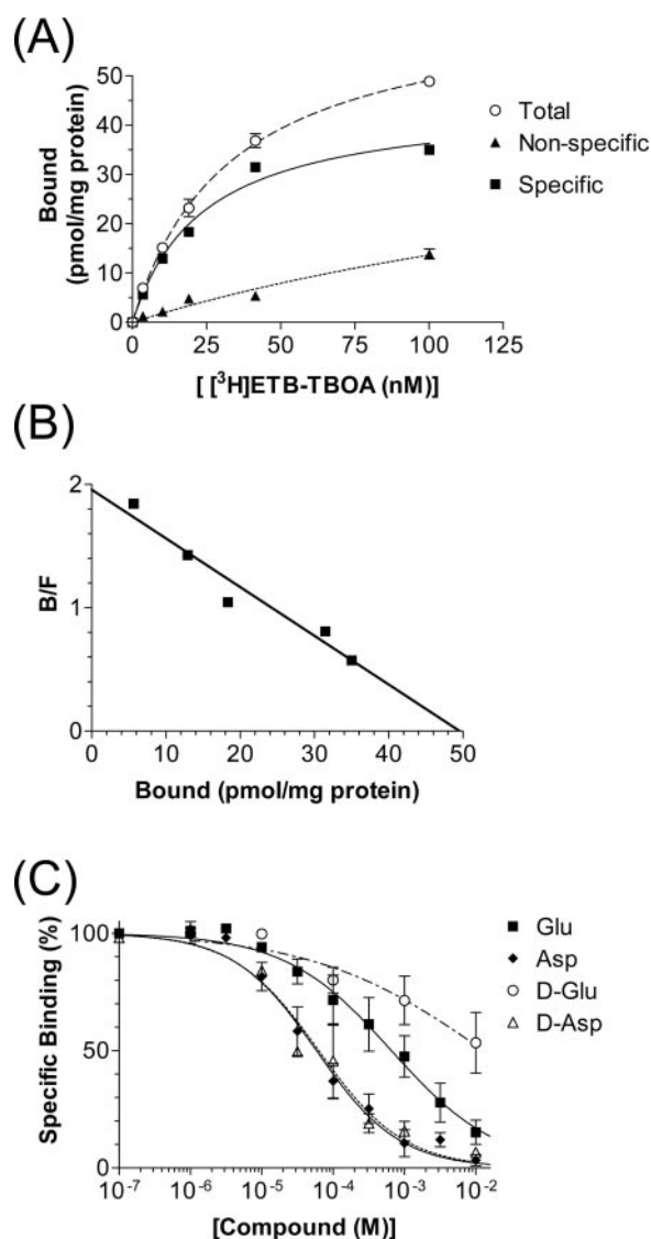
Fig. 3. [ ^3\text{H} ]ETB-TBOA binding to rat brain crude membranes. A, representative saturation plot; B, its Scatchard analysis. C, inhibition of [ ^3\text{H} ]ETB-TBOA binding by EAAT substrates. Nonspecific binding was determined in the presence of 10 \mu\text{M} TFB-TBOA. Data represent mean \pm S.E.M. of at least three separate experiments.
