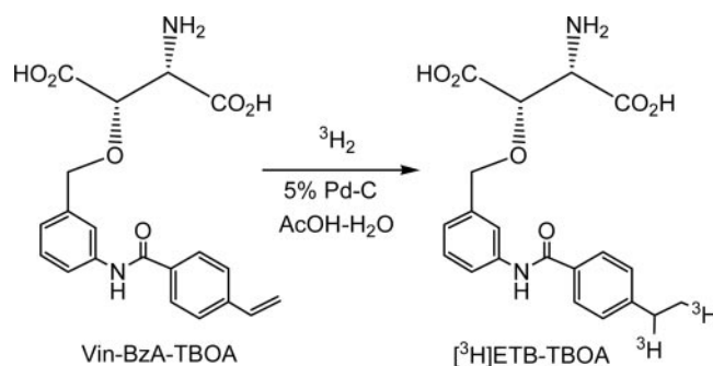
Fig. 1. Synthesis of [^3\text{H}]\text{ETB-TBOA} from Vin-BzA-TBOA.
