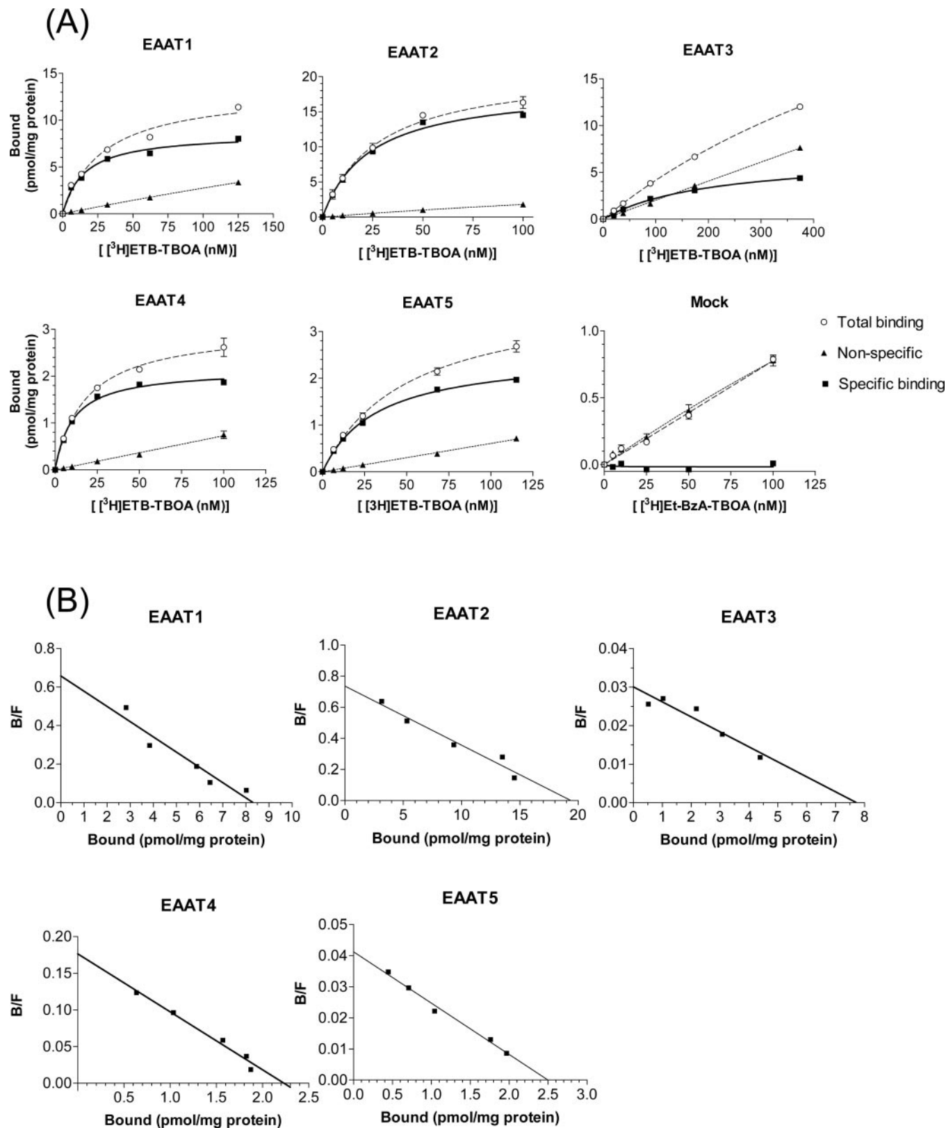
Fig. 4. [^3\text{H}]\text{ETB-TBOA} binding to EAAT-expressing COS-1 cell membranes. A, representative saturation plots. Specific binding was detected in EAAT-expressing cell membranes but not in vector-expressing cell membranes (mock). B, Scatchard analysis of the saturation data.
